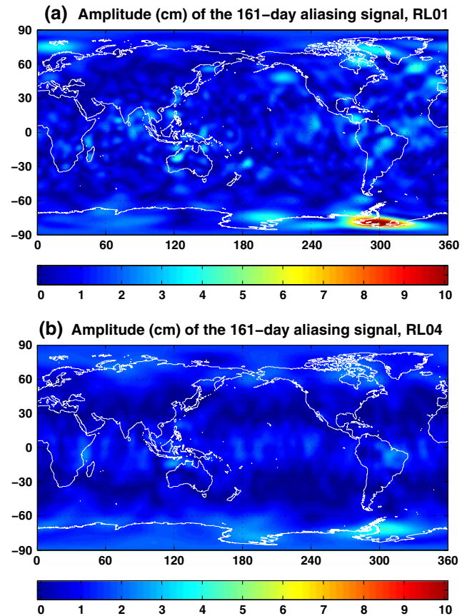
Fig. 1 a Least square fit amplitude (cm of equivalent water height) of the 161-day S 2 alias from the 53 monthly GRACE solutions in RL01. b As in a but for RL04
