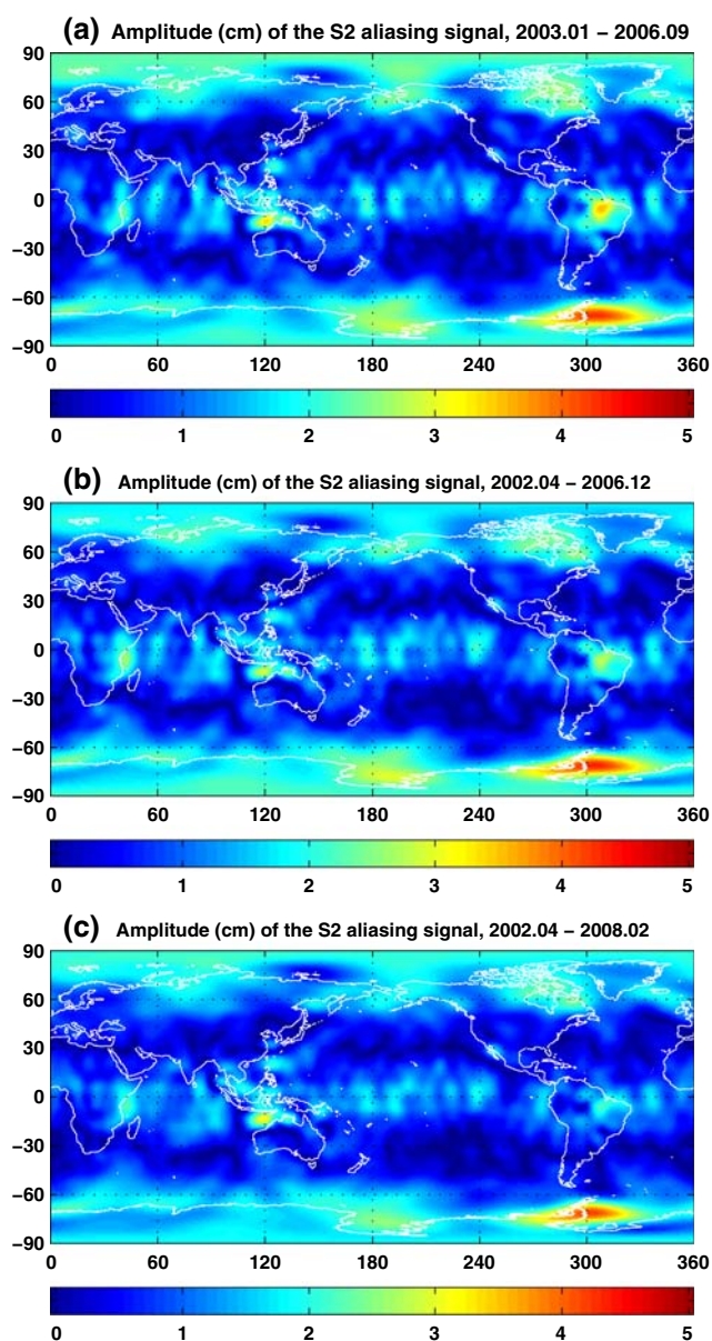
Fig. 8 Least square fit amplitude (cm of equivalent water height) of the 161-day alias from CSR RL04 monthly solutions for 3 different periods a January 2003–September 2006, b April 2002–December 2006, and c April 2002 – February 2008
