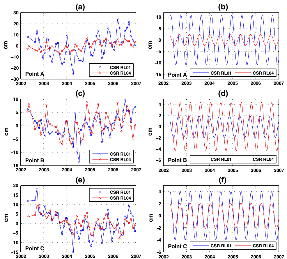
Fig. 4 Left panels (a, c, and e) compare apparent mass change time series (RL01 and RL04) at points (A, B, and C) marked by crosses in Figs. 2a, b, and 3a, respectively. Right panels (b, d, and f) compare 161-day amplitudes for RL01 and RL04 at points (A, B, and C)
