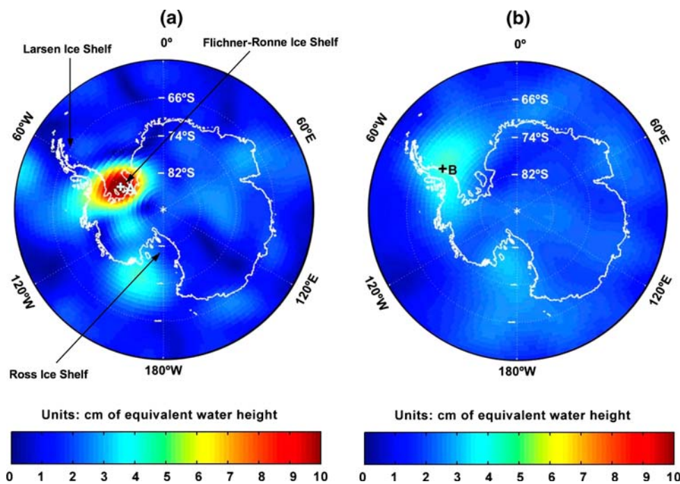
Fig. 2 a Detailed view of the Antarctic of the amplitude of the 161-day alias in RL01. b As in a but for RL04
