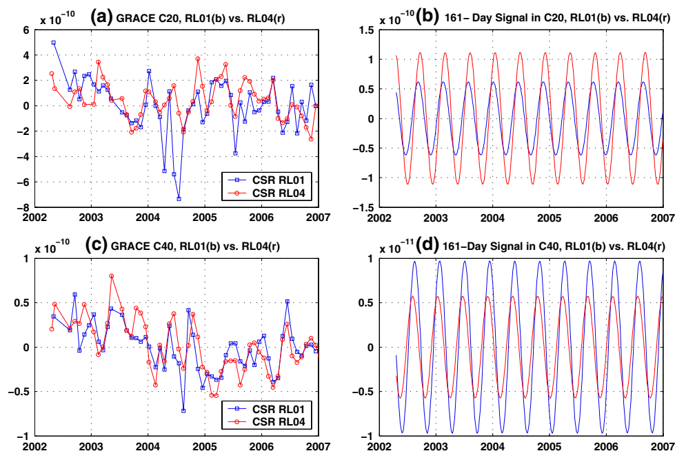
Fig. 5 Left panels compare GRACE RL01 and RL04 solutions of a C_{20} and c C_{40} . Right panels ( b , d ) compare 161-day amplitudes for RL01 and RL04 solutions of C_{20} and C_{40} . GRACE GAC atmospheric and oceanic averages are not restored
