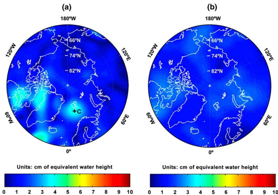
Fig. 3 a Detailed view of the Arctic of the 161-day alias for RL01. b As in a but for RL04
