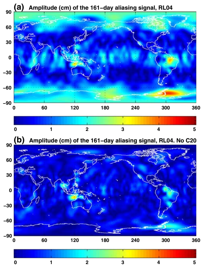
Fig. 6 a Amplitudes (cm of equivalent water height) of the 161-day alias signal from 53 CSR RL04 monthly solutions with C_{20} included (same as Fig. 1b, but different color scale). b As in a , but with C_{20} excluded
